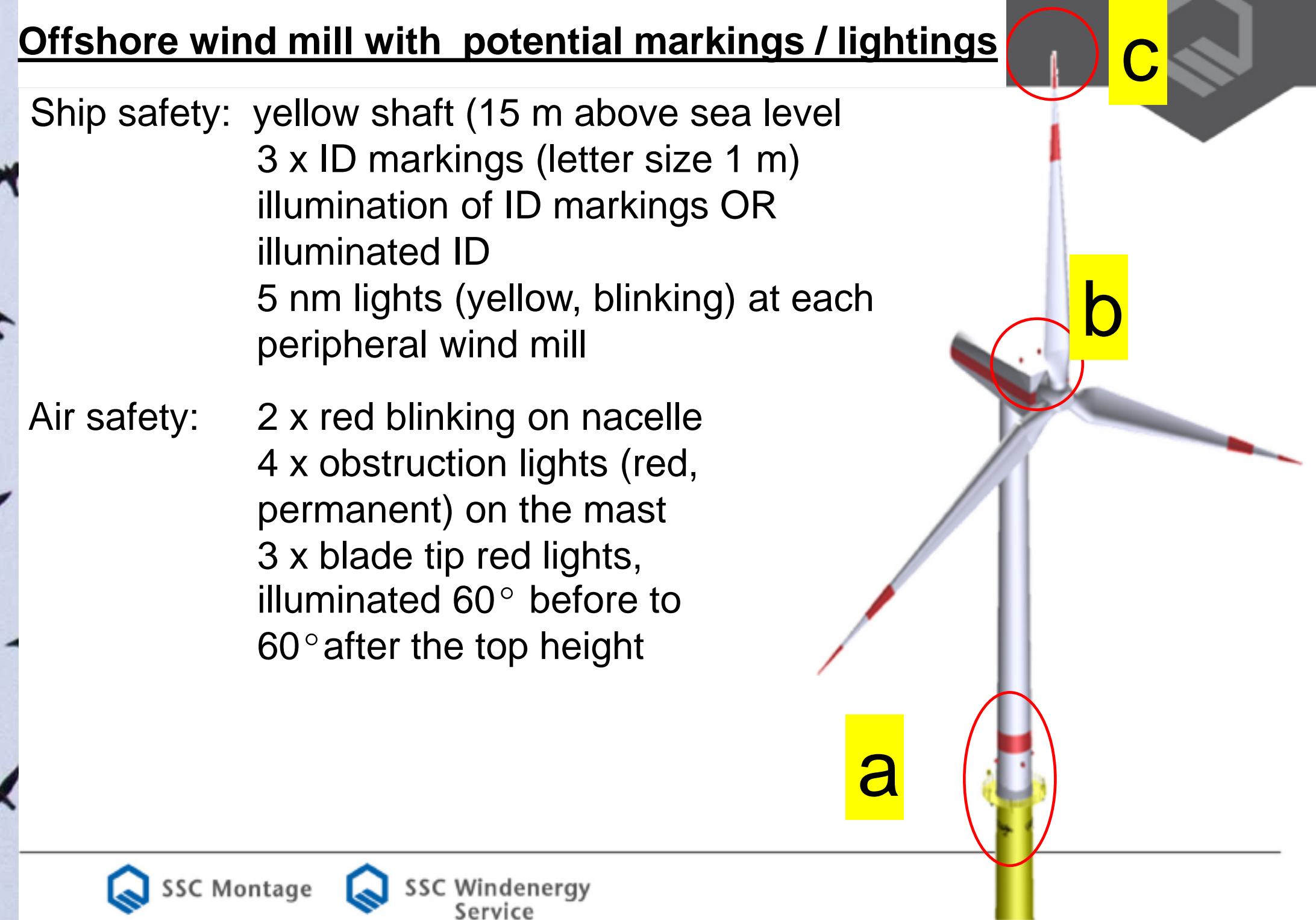
Fig. 1: Obstruction lighting on a model offshore windmill > 150 m in German waters; for smaller wind mills the "4 x obstruction lights" and "blade tip red lights" are not mandatory.
