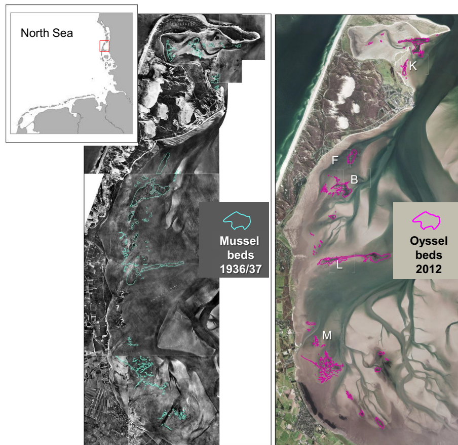
Fig. 2. Aerial photographs of northern Sylt with tidal flats exposed at low tide in 1936/37 with mussel beds (blue contours) and in 2012 with beds composed of mussels and oysters ("oyssel" beds, red contours). K, Königshafen; F, oysterfarm; B, Blidsel; L, Leghörn; M, Munkmarsch.
